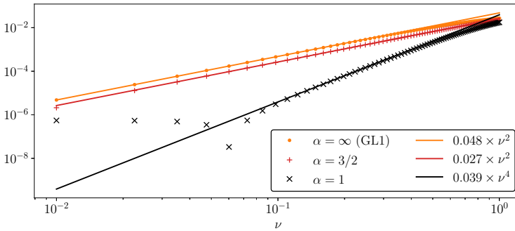
Fig. 5 Deviation of the effective diffusion coefficient from its limiting value as \nu \rightarrow 0 . For \alpha = 1 , we observe that the data are not aligned with the straight line for small values of \nu , which we attribute to round off errors
