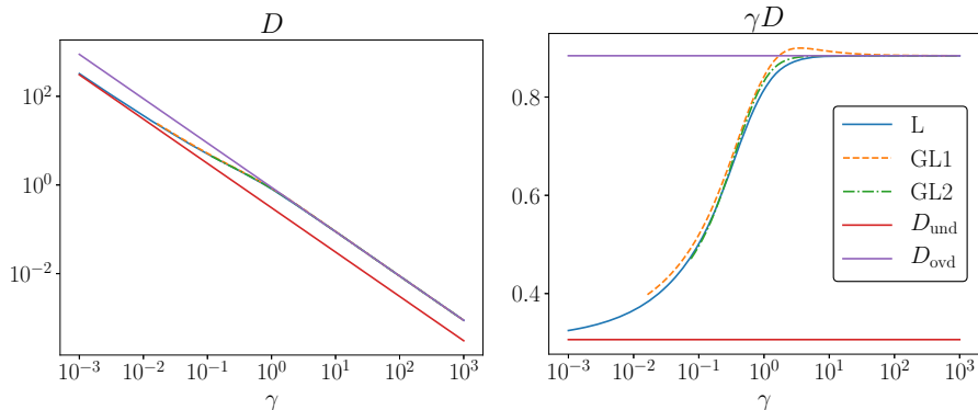
Fig. 3 Diffusion coefficient as a function of \gamma , for the parameters \nu = 1 (for the models GL1 and GL2) and \alpha = 1 (for GL2). We observe that, for values of \gamma in the range [1, 10] , the GL1 diffusion coefficient is slightly larger than D_{\text{ovd}}/\gamma
