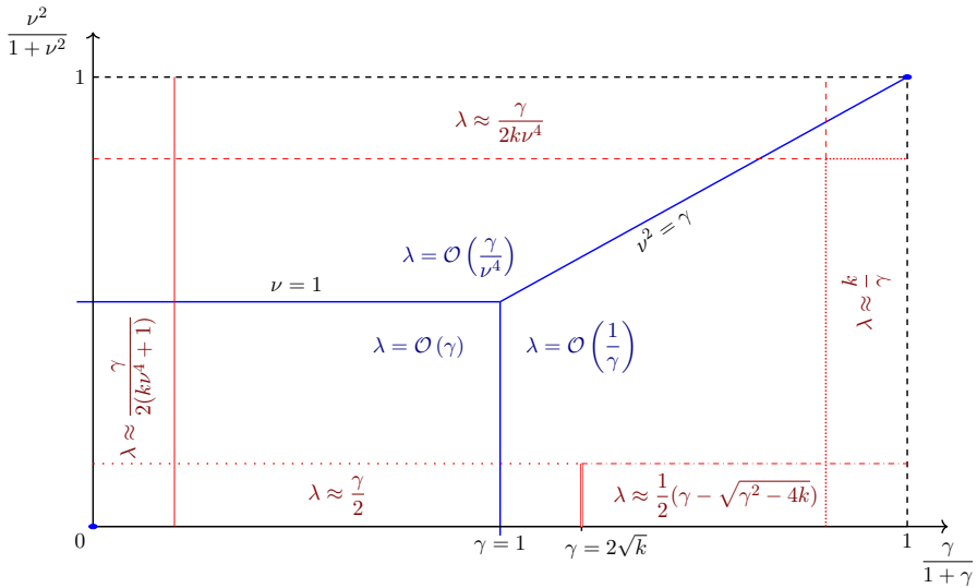
Fig. 2 Schematic illustration of the scaling of the exponential decay rate \lambda in L_0^2(\mu) . The general estimate, implied by (2.11) and valid under the general Assumption 2.1, is illustrated in blue. The behavior of the exponential growth bound in the particular case of the quadratic potential V(q) = k\frac{q^2}{2} is depicted in red. In this context, the symbol \approx means that the relative error is arbitrarily close to zero in the corresponding limit
