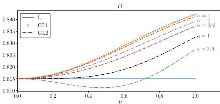
Fig. 4 Effective diffusion coefficient against \nu , whose square encodes the characteristic time of the auto-correlation function of the noise, for fixed values \beta = \gamma = 1
