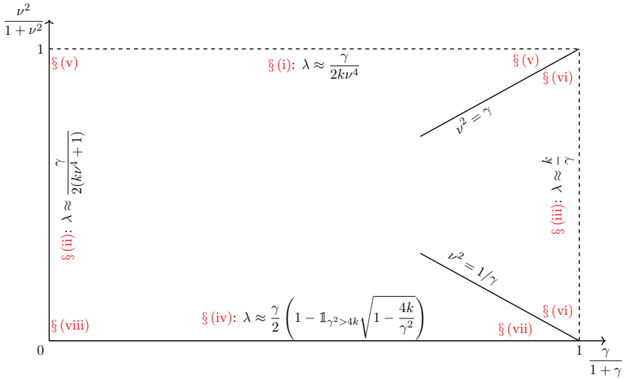
Fig. 7 Illustration of the different limits considered in this appendix. The joint limit \gamma \rightarrow \infty and v \rightarrow \infty with \gamma/v^2 bounded from above and below, as well as the joint limit \gamma \rightarrow \infty and v \rightarrow 0 with \gamma v^2 bounded from above and below, are omitted for conciseness
