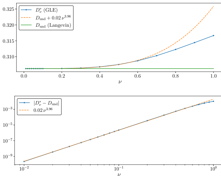
Fig. 6 Comparison between the effective diffusion coefficients (multiplied by \gamma ) for the Langevin and the generalized Langevin dynamics in the underdamped limit, in linear (top) and logarithmic (bottom) scales
