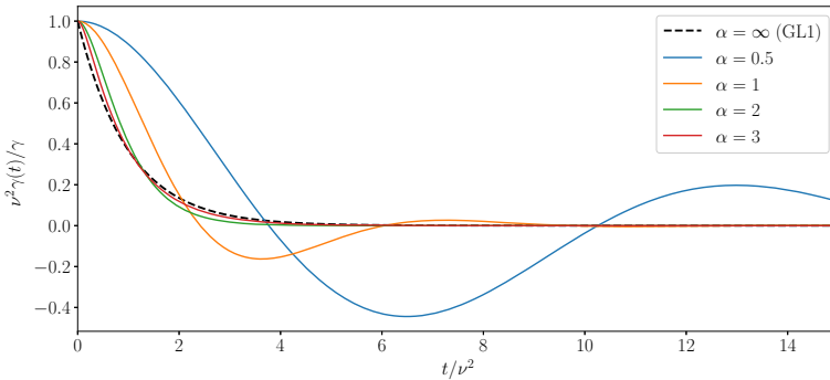
Fig. 1 Memory kernels associated with models GL1 and GL2 (with time rescaled by a factor v^{-2} and memory kernel rescaled by a factor v^2/\gamma in order to have shapes independent of the choices of \gamma, v )
